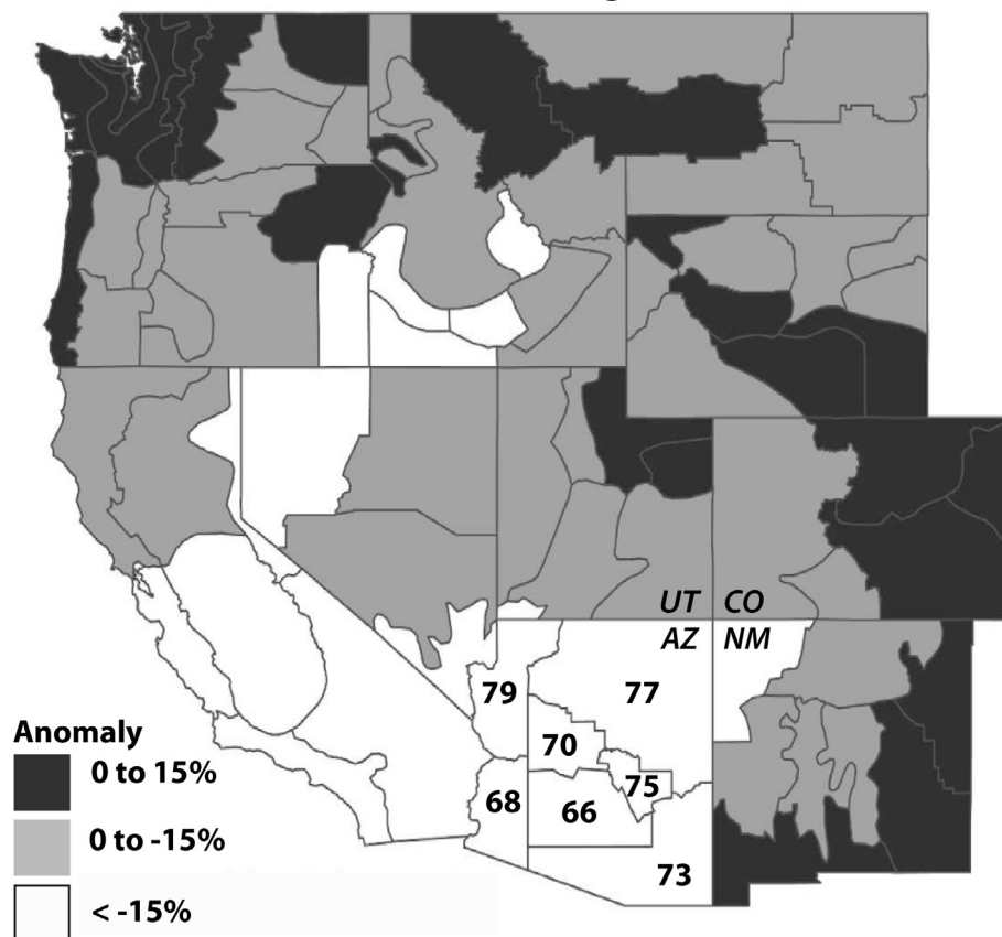
Figure 2. Winter precipitation for all December–March periods for each climate division in the West between 1925 and 1998 in which ENSO was neutral (defined as when the SST average over the Niño 3.4 region falls between -0.5 and 0.5 degrees Celsius) and the PDO was negative. Results from this analysis show that 68 of 84 climate divisions generally experienced below-average precipitation. The map is modified from Goodrich (2007) and the numbers in Arizona correspond to the percent of average winter precipitation calculated for each of the state's climate divisions during the same periods noted above; the numbers were obtained from Goodrich (2004).
