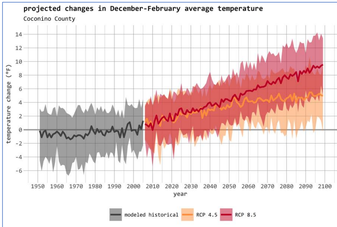
Figure A4: Downscaled model projections of average temperature for Coconino County during December – February.
