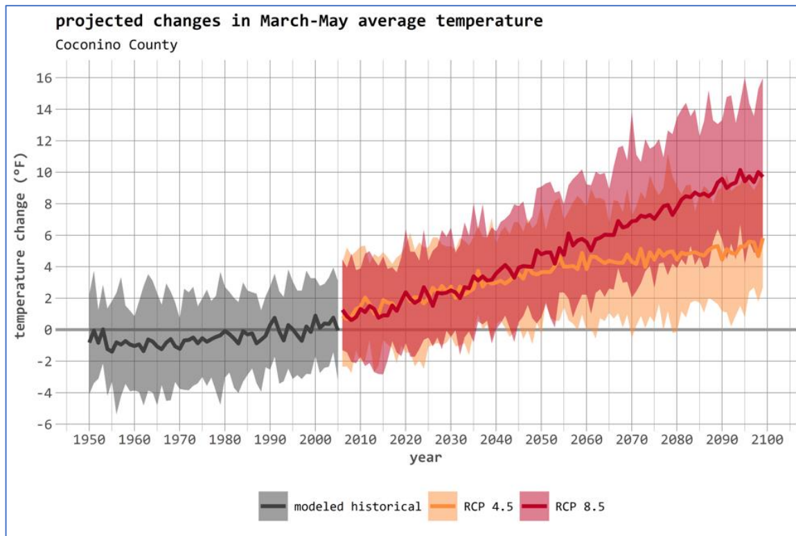
Figure A9: Downscaled model projections of average temperature for Coconino County during March – May.
