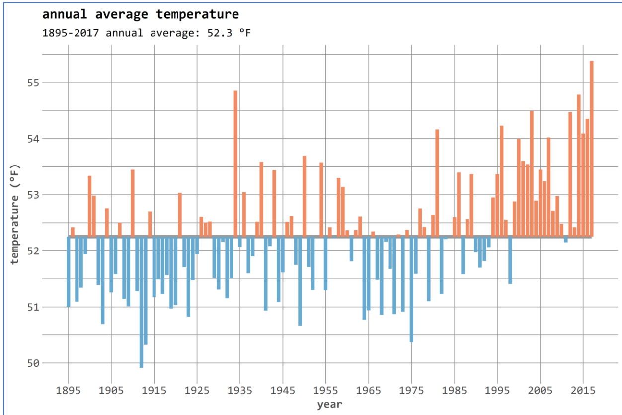
Figure 7: Average annual temperatures for Coconino County from 1895 – 2017.
