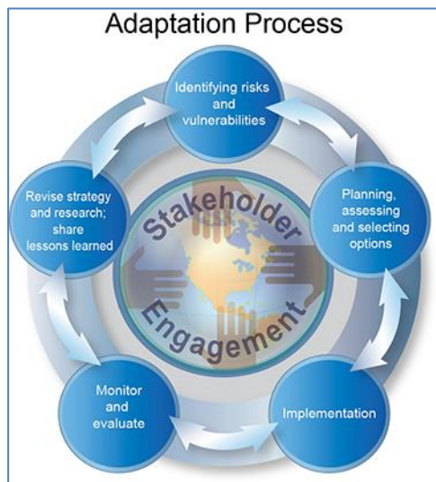
Figure 6: The Adaptation Process. Source http://nca2014.globalchange.gov/report/response-strategies/adaptation
