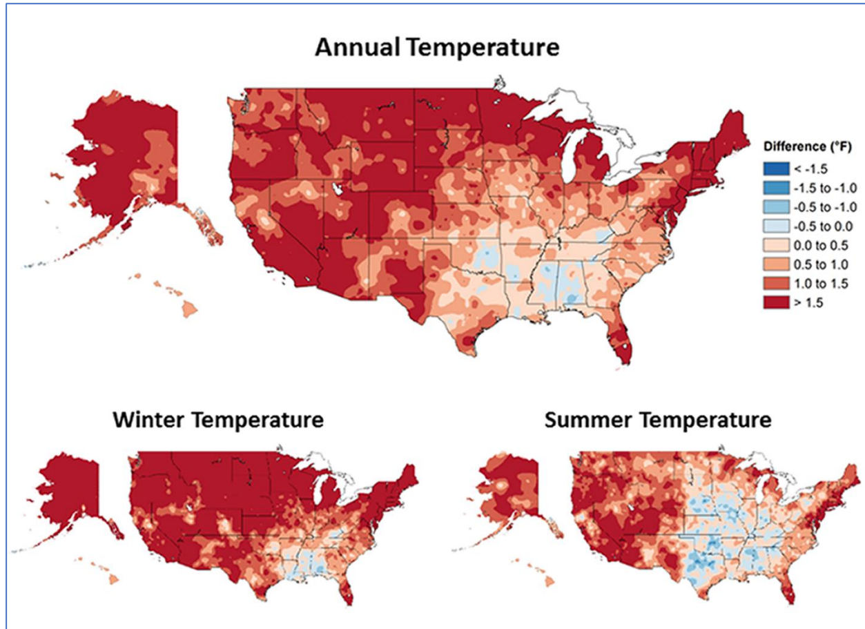
Figure 2: Observed temperature changes in the U.S. comparing the current period (1986 – 2016) to the period 1901–1960. The darker the color, the greater the difference between 1901–1960 and 1986 - 2016. Source: Climate Science Special Report: https://science2017.globalchange.gov/ .
