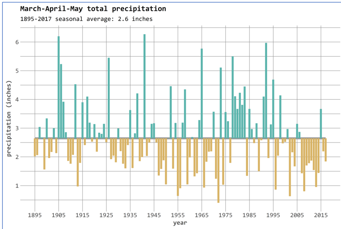
Figure A8: Total precipitation during March – May for Coconino County from 1895 – 2017.
