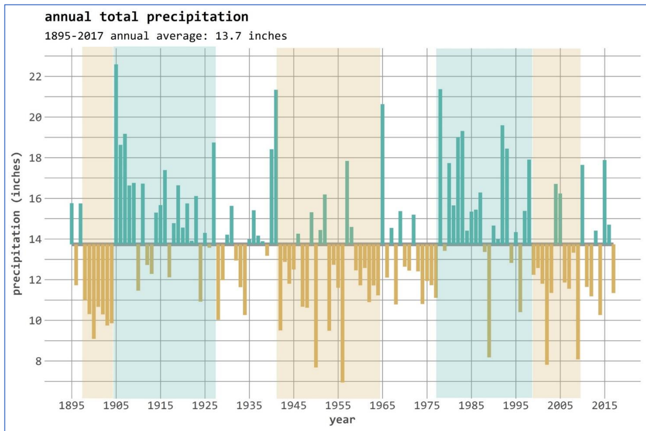
Figure 9: Average annual precipitation for Coconino County 1895 - 2017
