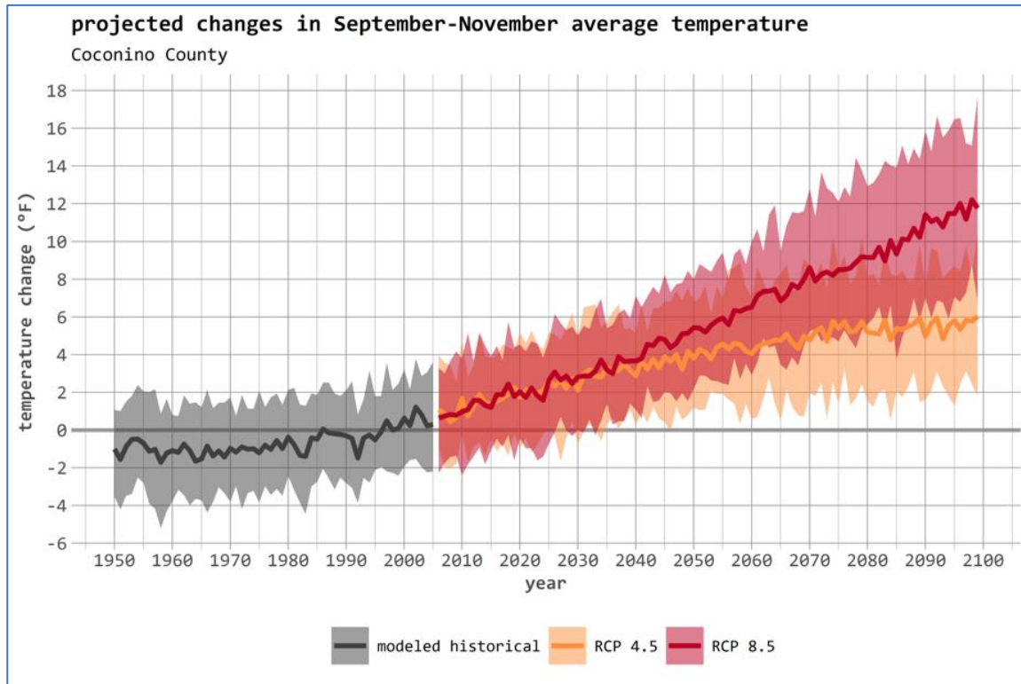
Figure A19: Downscaled model projections of average temperature for Coconino County during September – November.
