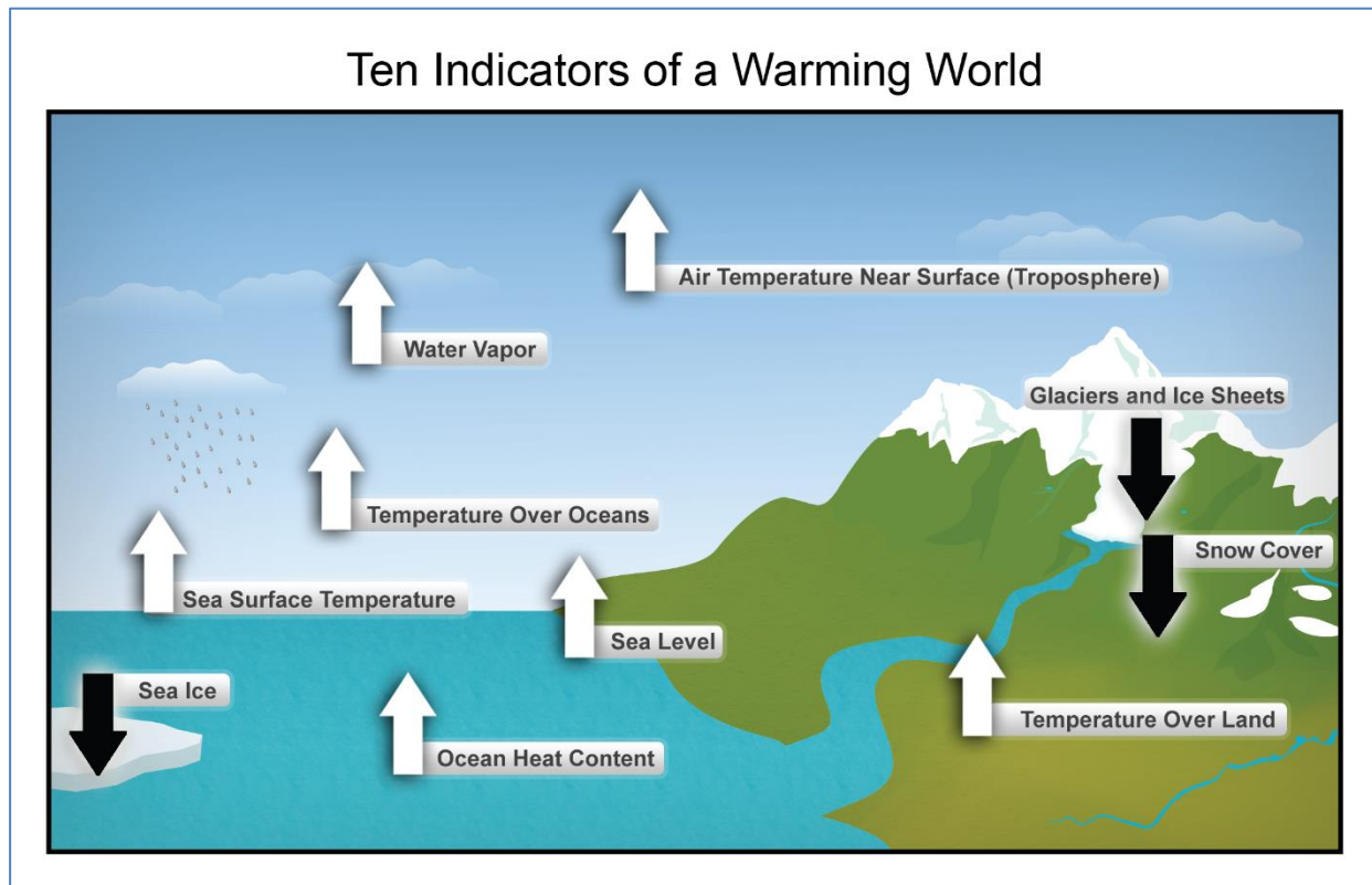
Figure 1: Observed indicators of a warming world. White arrows indicate increasing trends. Black arrows indicate decreasing trends. Source: http://nca2014.globalchange.gov/report/our-changing-climate/observed-change#tab2-images .
