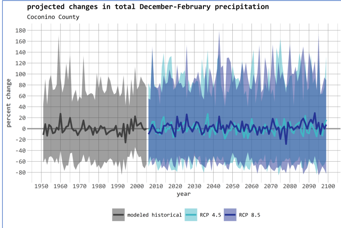
Figure A5: Downscaled projections of total precipitation for Coconino County during December – February.
