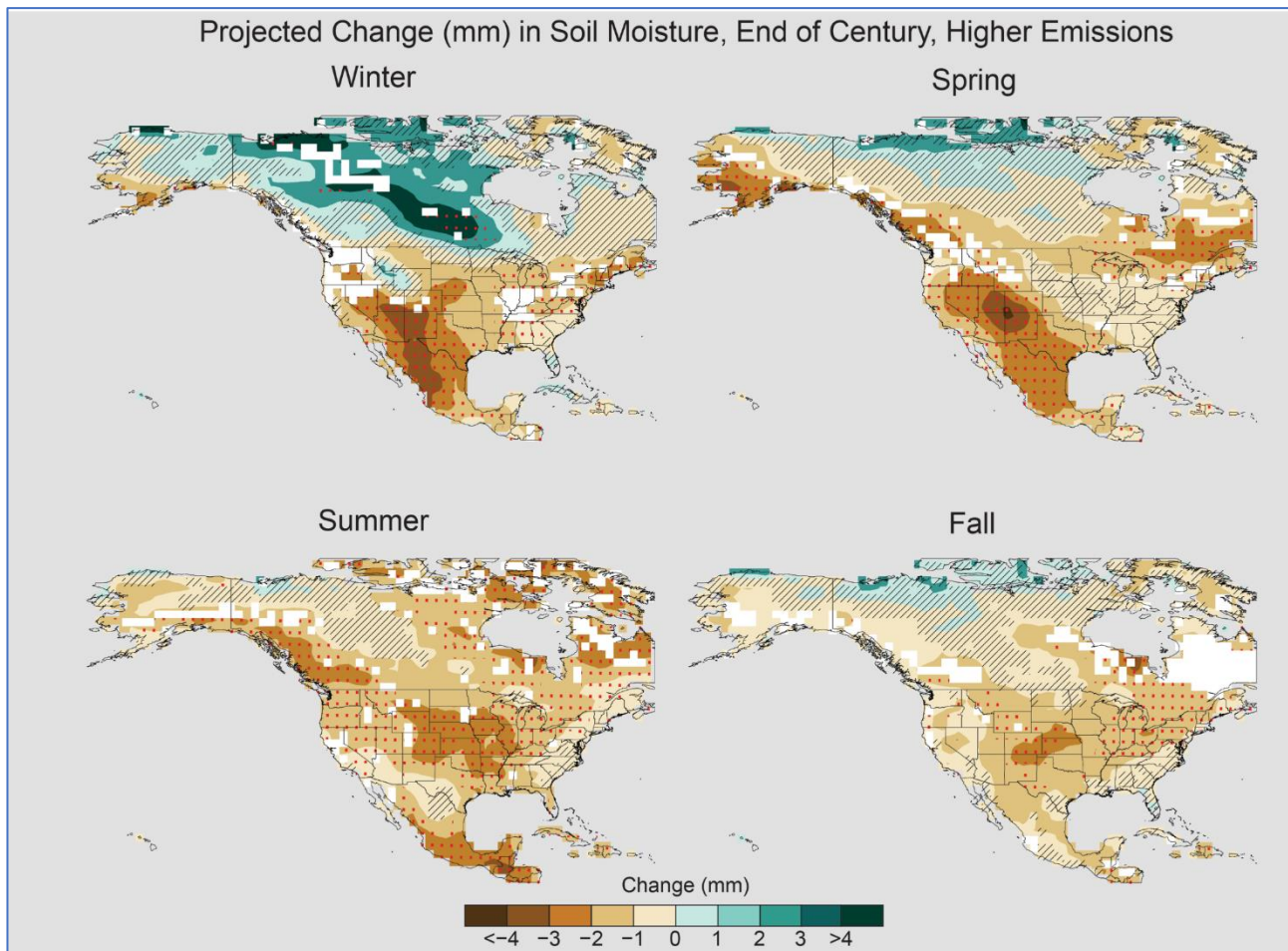
Figure 18: Projected changes in soil moisture by 2100 using the high emissions scenario. Source: https://science2017.globalchange.gov/chapter/8/
