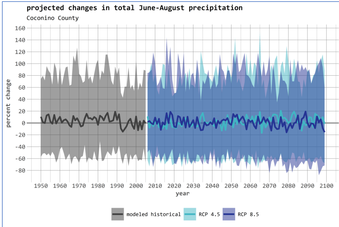
Figure A15: Downscaled projections of total precipitation for Coconino County during June – August.
