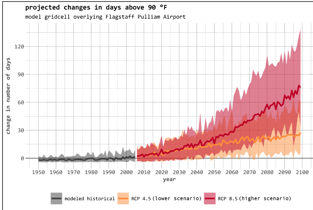
Figure 19: Projected changes in number of days in which maximum temperatures reach 90° F in Flagstaff.
