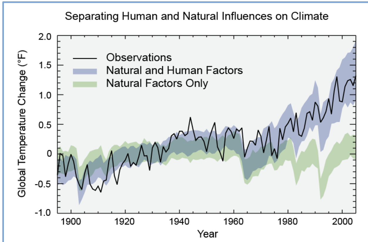
Figure 5: Results from a model experiment to compare natural warming factors with observed temperature changes since 1895. Source: Third National Climate Assessment, http://nca2014.globalchange.gov/report/our-changing-climate/observed-change#tab2-images
