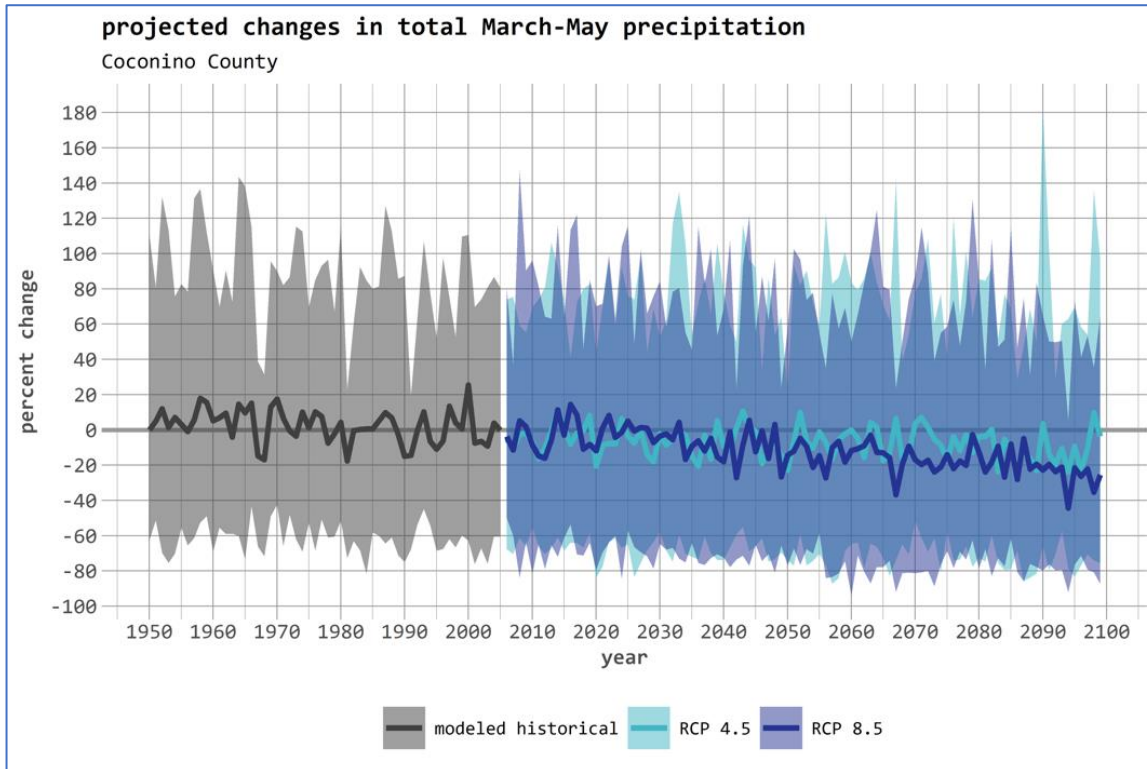
Figure A10: Downscaled projections of total precipitation for Coconino County during March – May.
