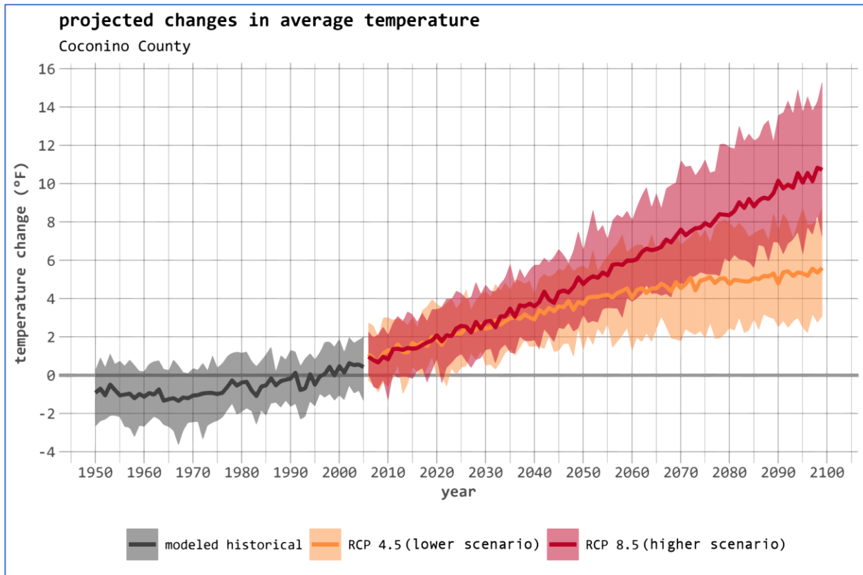
Figure 16: Downscaled model projections for Coconino County show a range of possible future temperature increases, from 3° F higher than the 1986–2005 average for RCP 4.5 (orange line), to 10° F higher for RCP 8.5 (red line).
