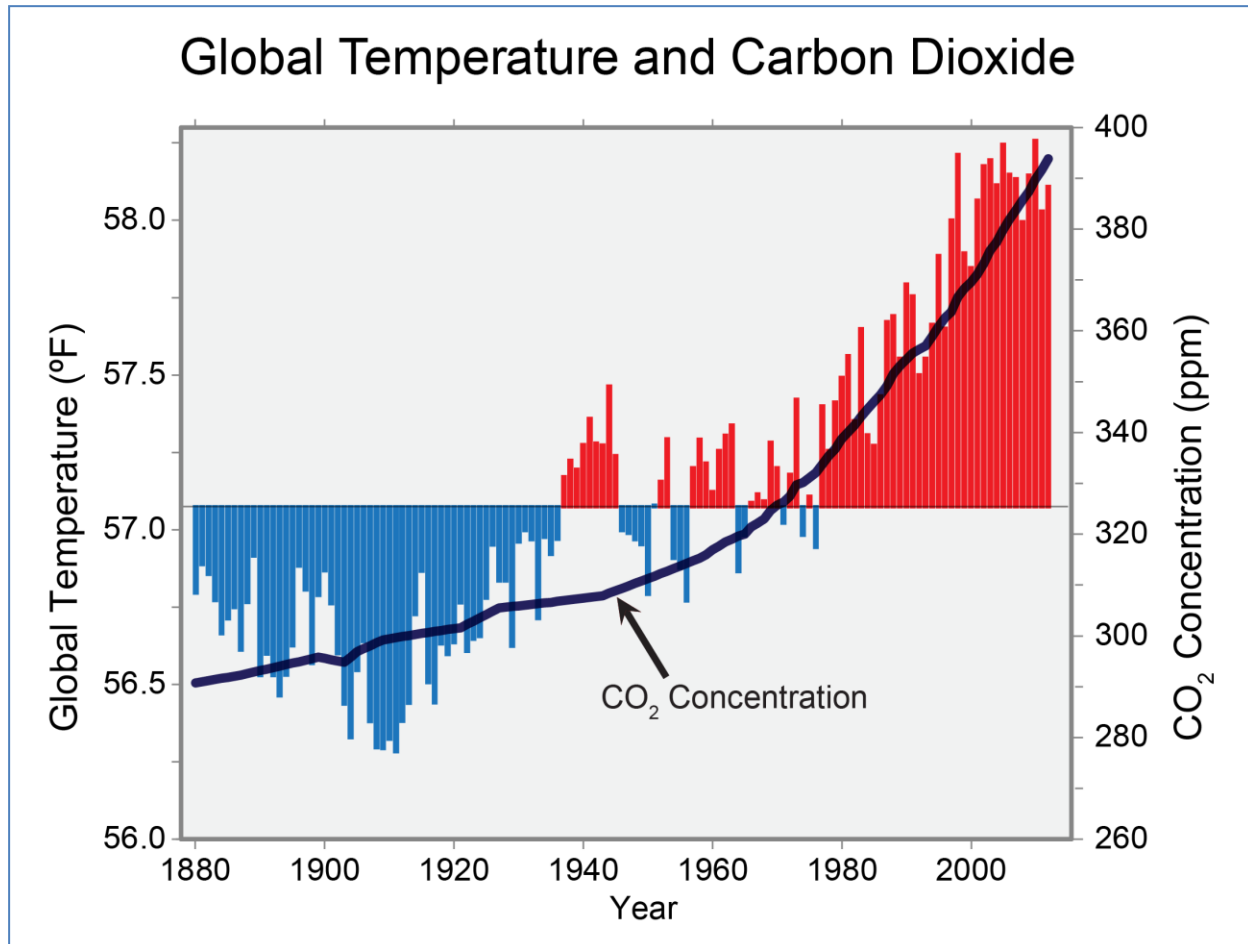
Figure 4: The corresponding rise in CO 2 and global temperatures. Source: http://nca2014.globalchange.gov/report/our-changing-climate/observed-change#tab2-images
