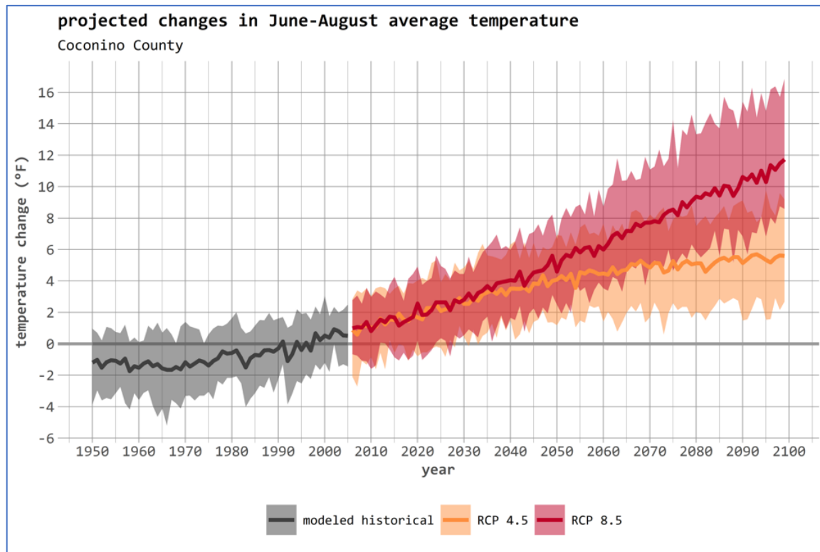
Figure A14: Downscaled model projections of average temperature for Coconino County during June – August.
